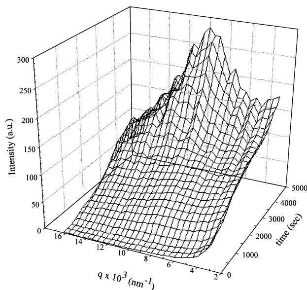
Fig. 9. A typical plot of intensity against time and q for melt mixed SMA/PMMAe (40/60) blends, obtained from a temperature jump experiment at 210°C.
